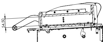
MMI-Standard height
