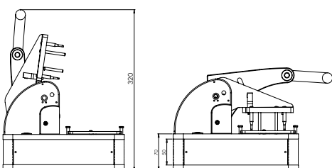
LHS2-Standardhöhe 50mm
